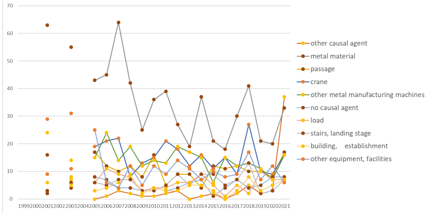
Transition of fatal and non-fatal accidents in small causal agents in code no. 011001 steel/iron/rolling products (1999-2021)
