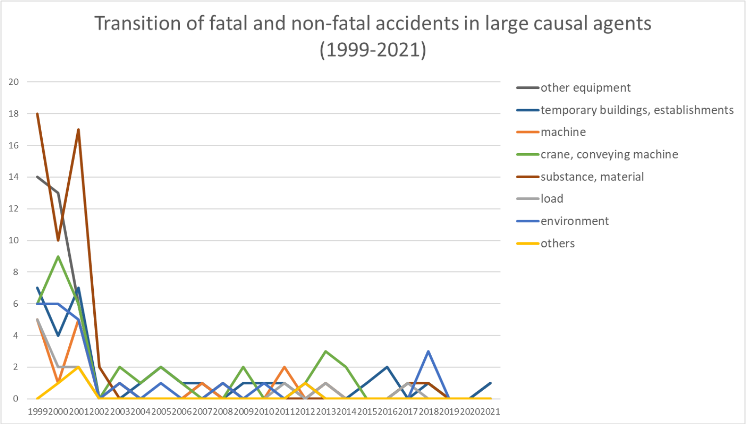
Transition of fatal and non-fatal accidents in large causal agents in code no. 0201 coal mining (1999-2021)
