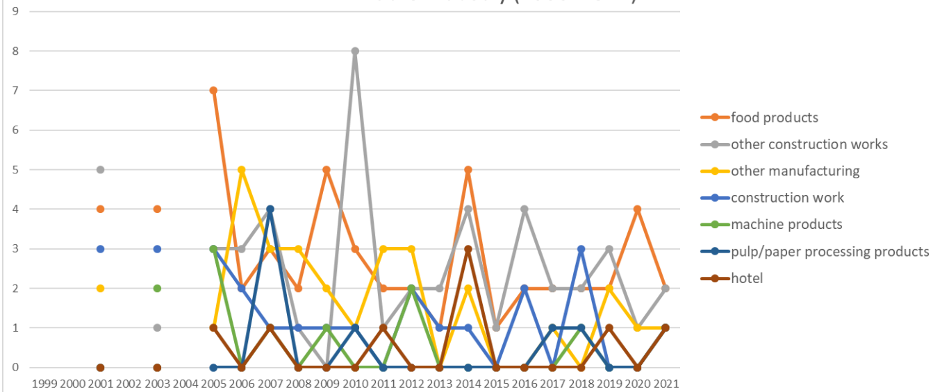
Transition of causal agents (Small) of fatal and non-fatal accidents as code no. 311 boiler in Middle Industry (1999-2021)
