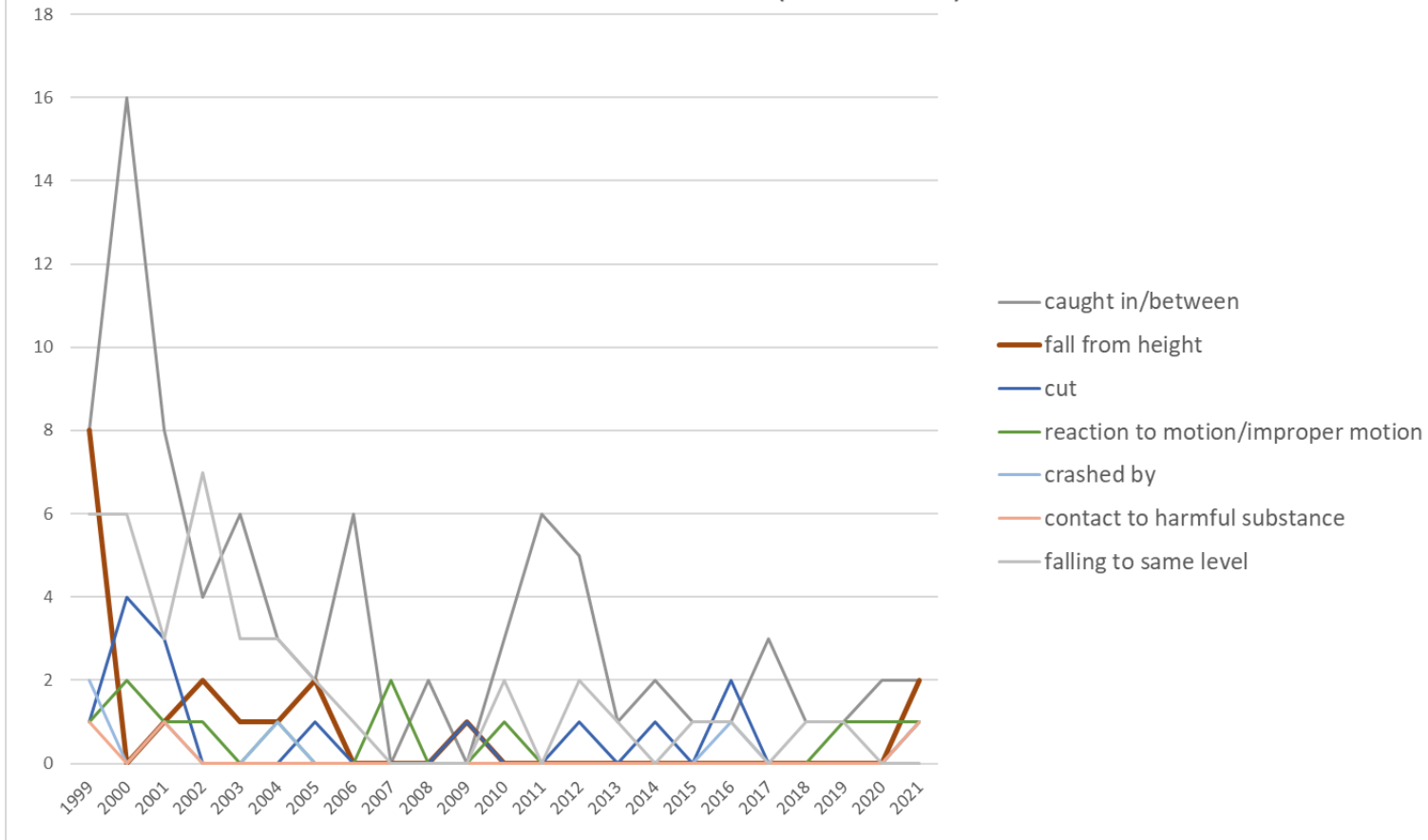
Transition of fatal and non-fatal accidents in type of accidents in code no. 010201 silk-reeling (1999-2021)
