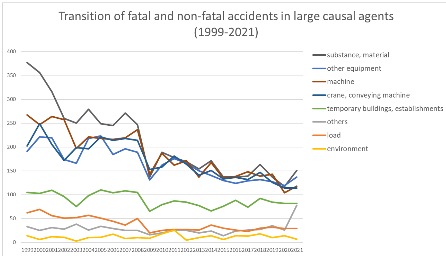
Transition of fatal and non-fatal accidents in large causal agents in code no. 0110 steel making (1999-2021)
