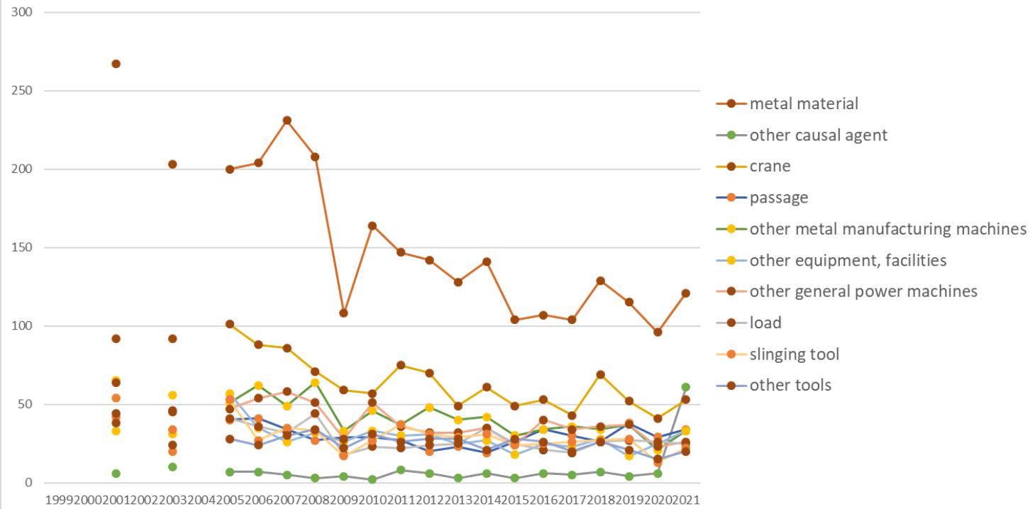
Transition of fatal and non-fatal accidents in small causal agents in code no. 0110 steel making (1999-2021)
