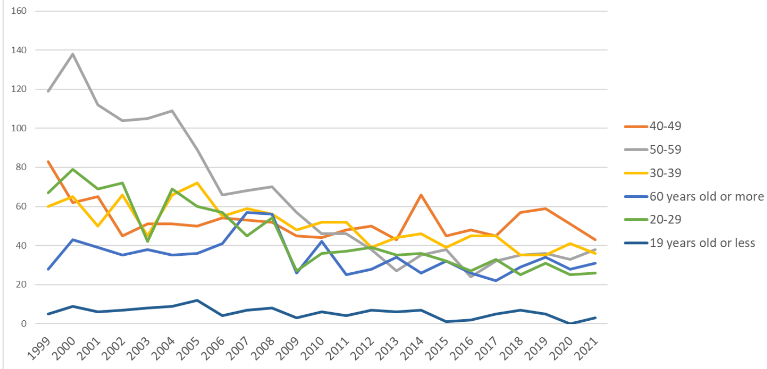
Transition of fatal and non-fatal accidents in workers ages in code no. 011009 other steel products (1999-2021)
