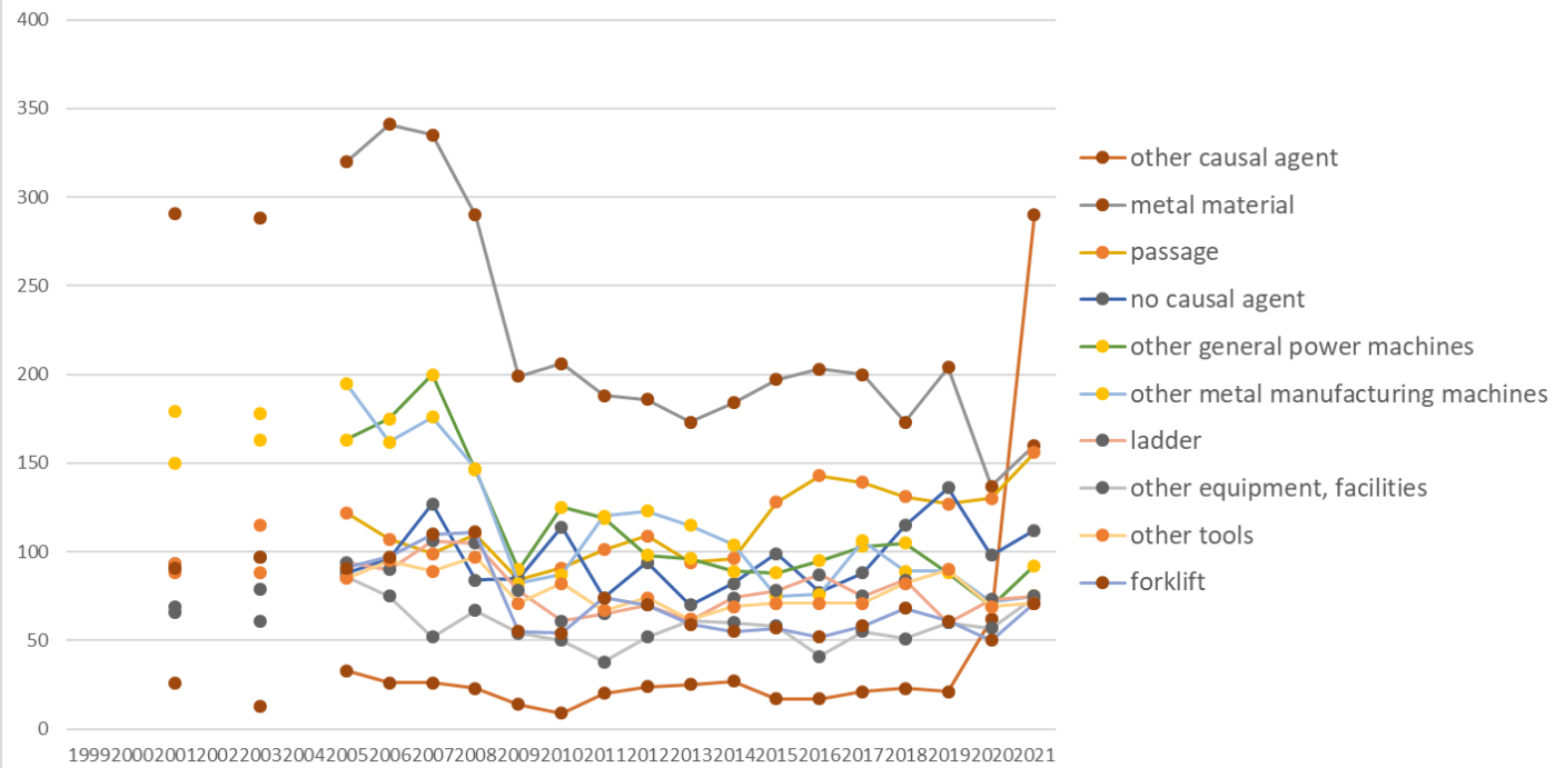
Transition of fatal and non-fatal accidents in small causal agents in code no. 0115 transport equipment products (1999-2021)
