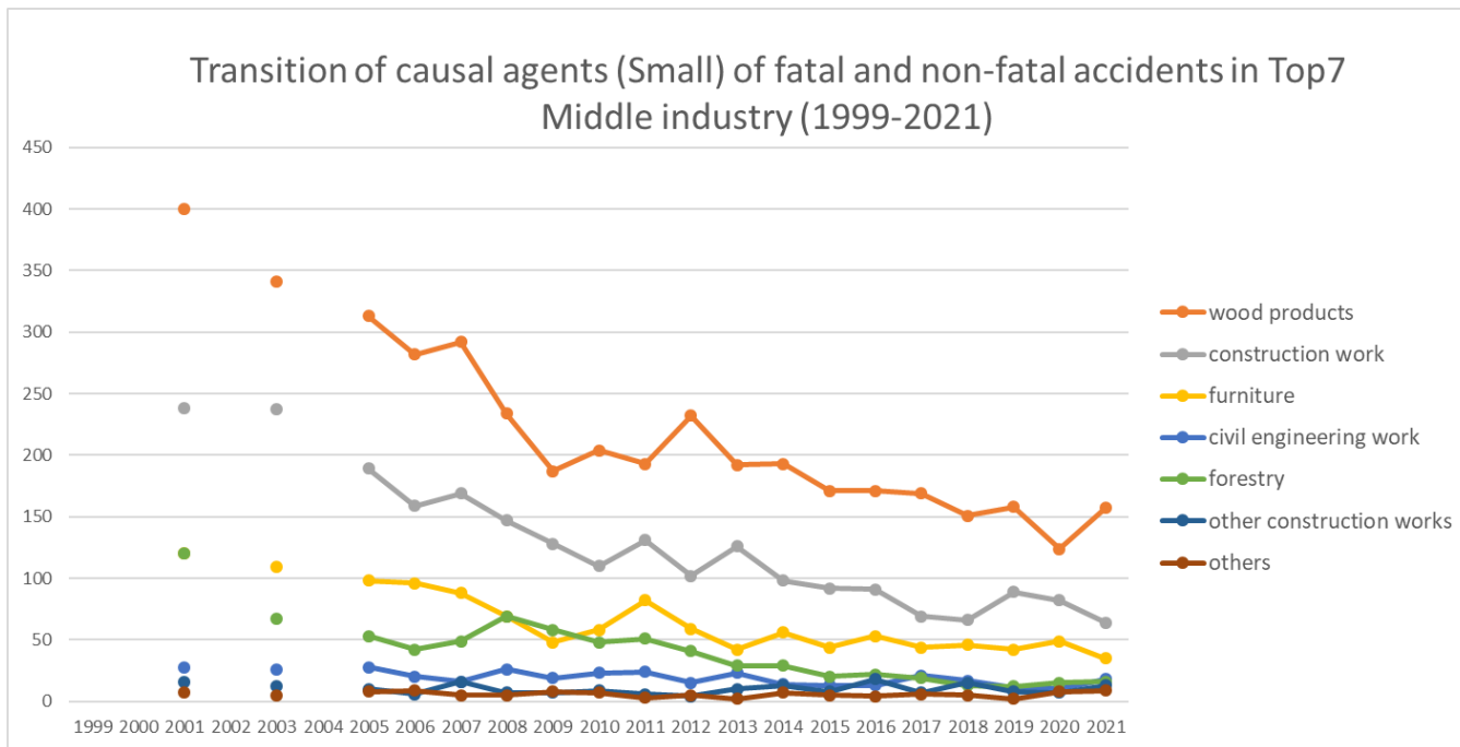
Transition of causal agents (Small) of fatal and non-fatal accidents as code no. 139 other woodworking machines in Middle Industry (1999-2021)
