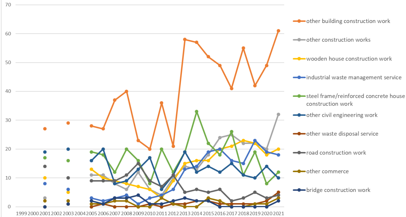
Transition of causal agents (Small) of fatal and non-fatal accidents as code no. 145 demolition machine in Small Industry (1999-2021)
