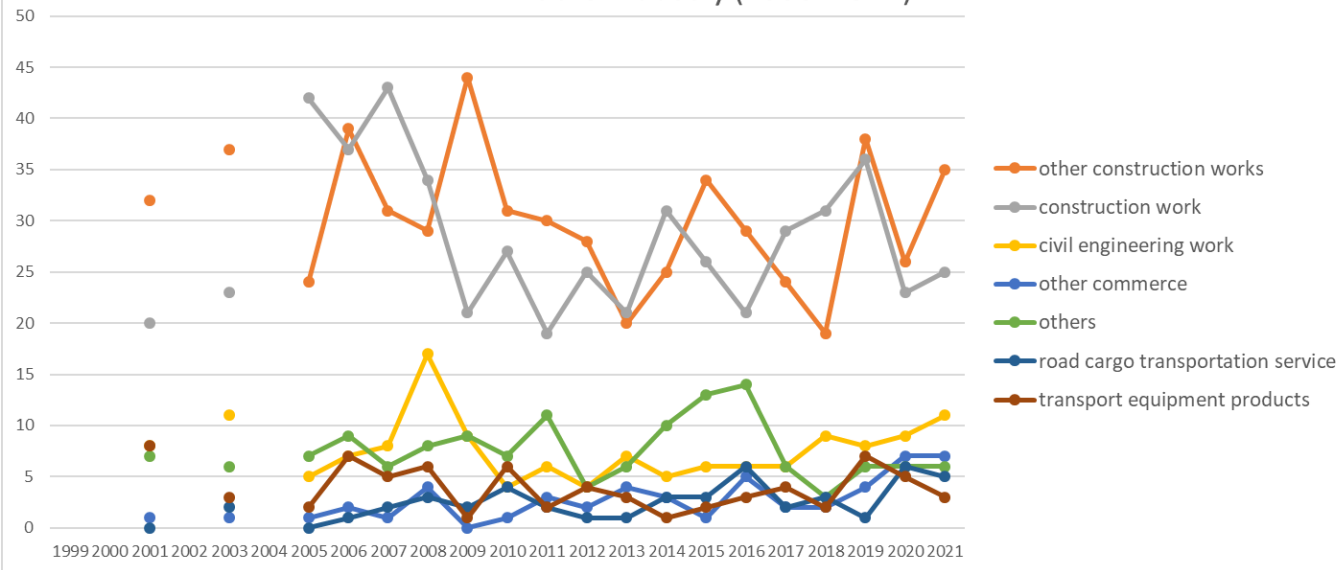
Transition of causal agents (Small) of fatal and non-fatal accidents as code no. 146 vehicle for high lift work in Middle Industry (1999-2021)
