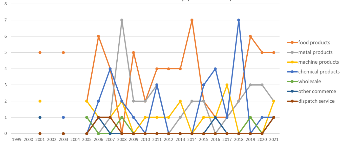
Transition of causal agents (Small) of fatal and non-fatal accidents as code no. 161 centrifugal machine in Middle Industry (1999-2021)
