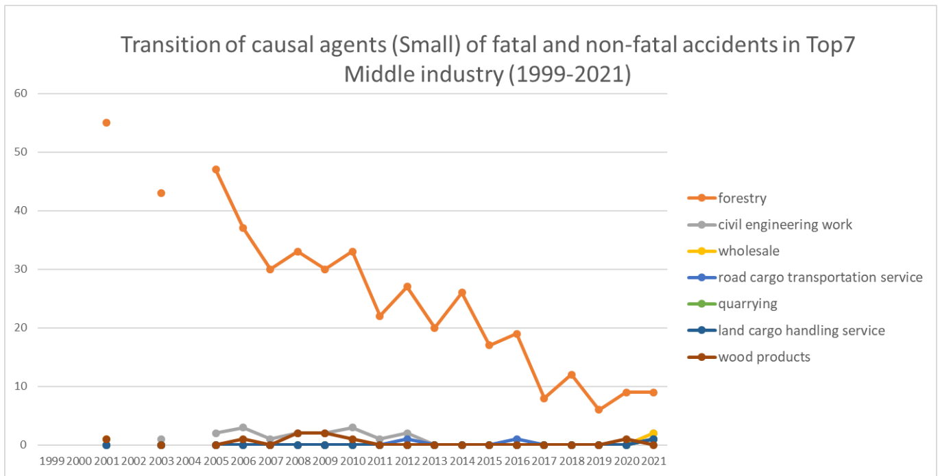
Transition of causal agents (Small) of fatal and non-fatal accidents as code no. 217 lumberyard equipment, logging cableway in Middle Industry (1999-2021)
