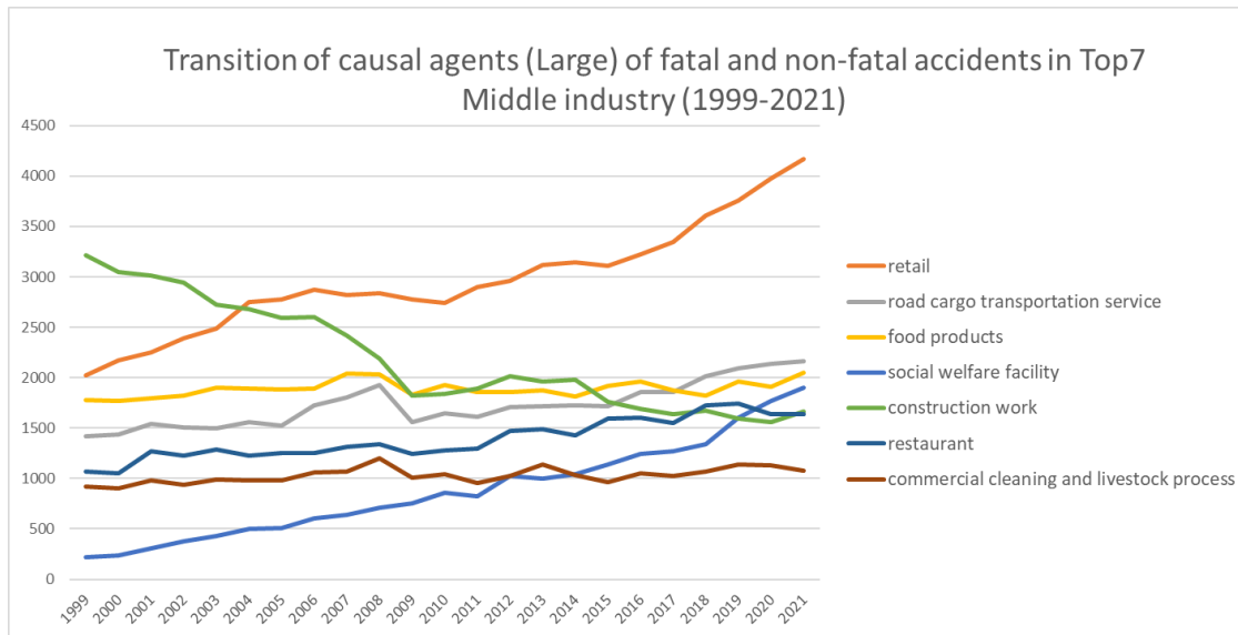
Transition of causal agents (Large) of fatal and non-fatal accidents as code no. 3 other equipment in Middle Industry (1999-2021)
