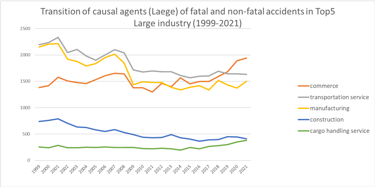
Transition of causal agents (Large) of fatal and non-fatal accidents as code no. 6 load in Large industry (1999-2021)
