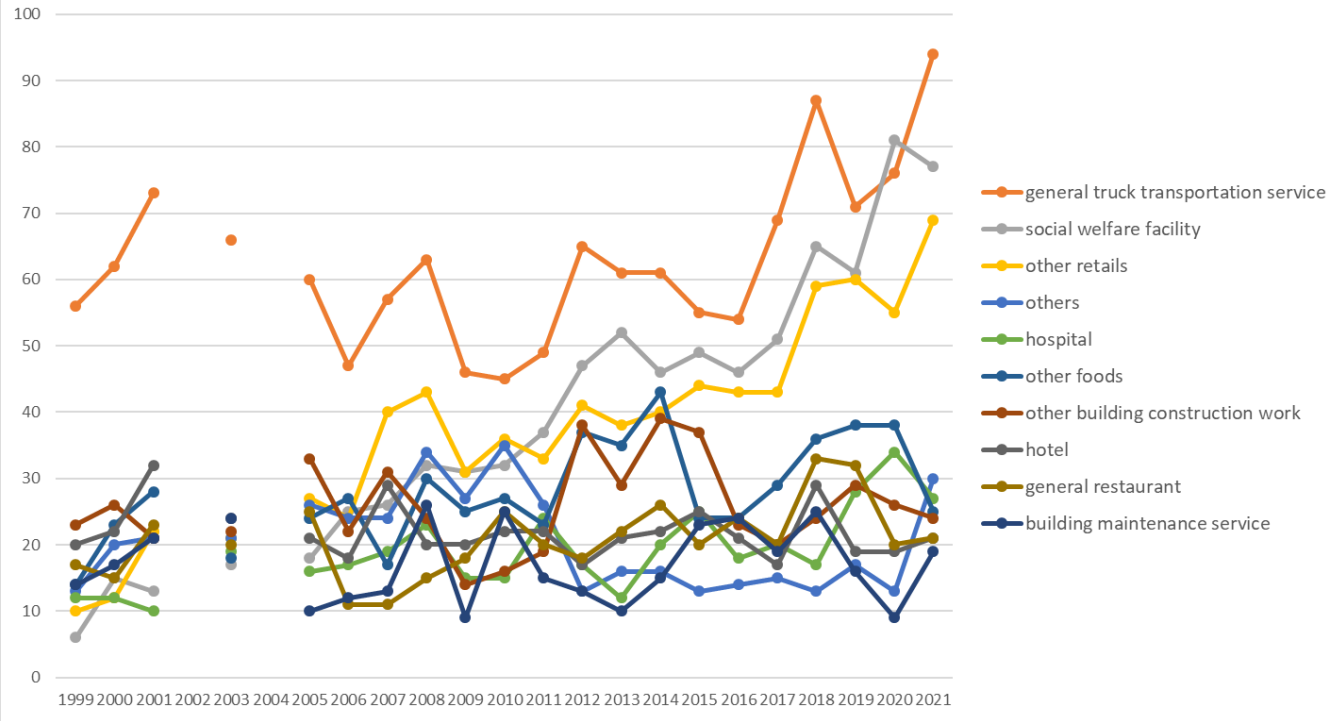
Transition of fatal and non-fatal accidents in Yamanashi in Small Industry (1999-2021)
