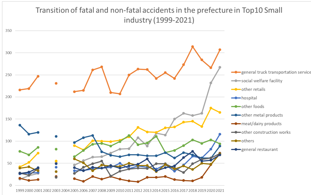
Transition of fatal and non-fatal accidents in Okayama in Small Industry (1999-2021)
