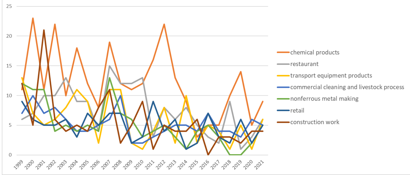
Transition of type of fatal and non-fatal accidents as code no. 14 explosion in Middle Industry (1999-2021)
