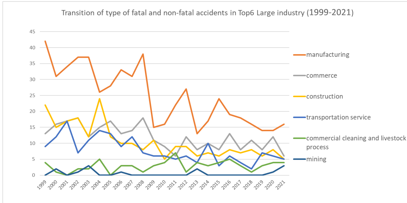
Transition of type of fatal and non-fatal accidents as code no. 15 burst in Large industry (1999-2021)
