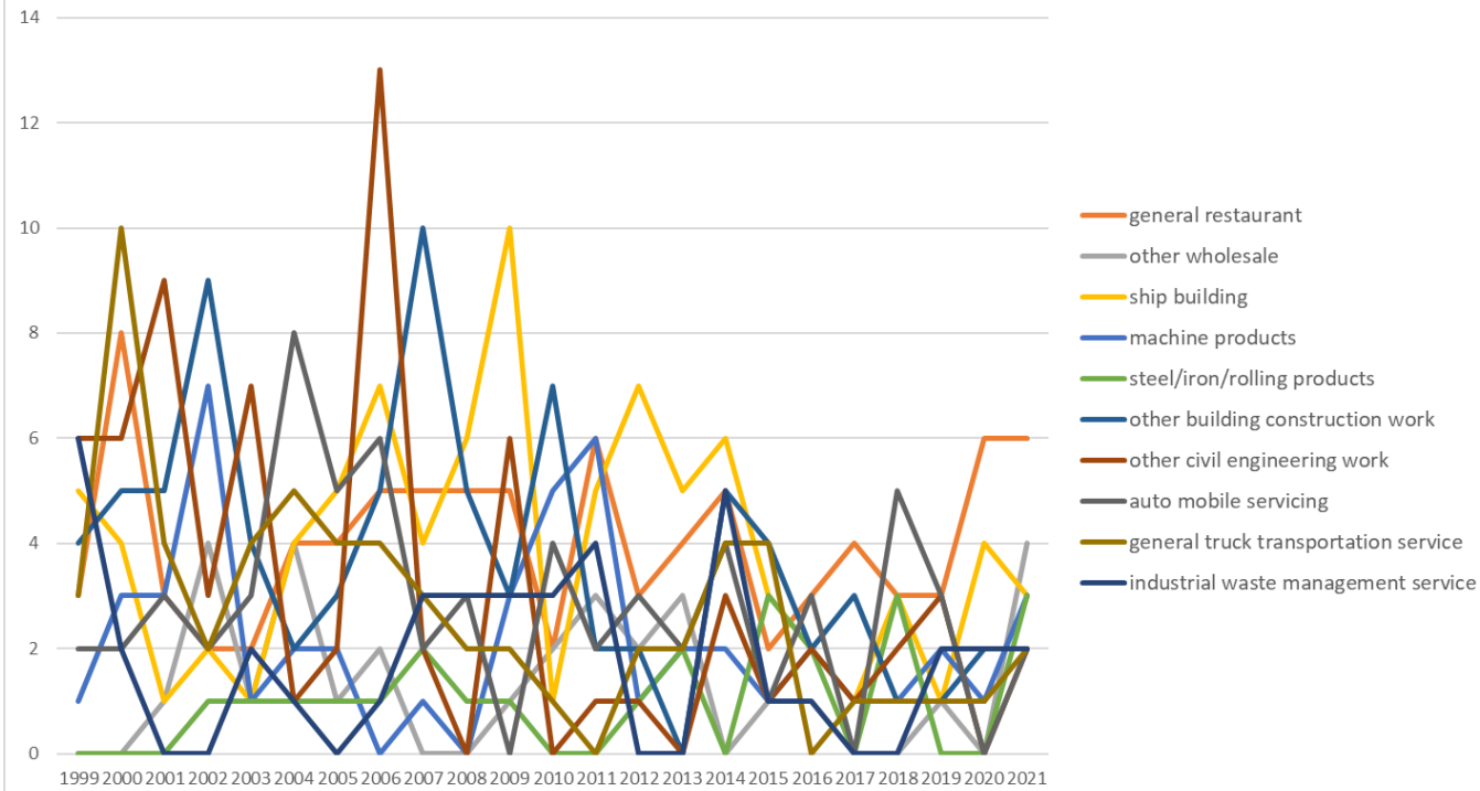
Transition of type of fatal and non-fatal accidents as code no. 16 fire in Small Industry (1999-2021)
