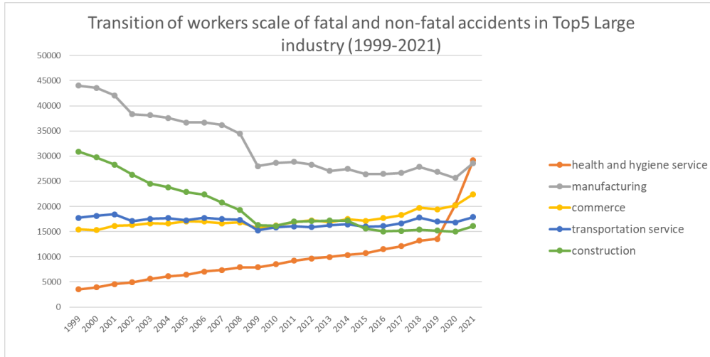
Transition of total workers scale of fatal and non-fatal accidents in Large industry (1999-2021)
