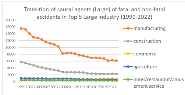
Transition of causal agents (Large) of fatal and non-fatal accidents as code no. 1 machine in Large industry (1999-2022)
