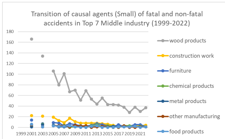
Transition of causal agents (Small) of fatal and non-fatal accidents as code no. 132 band sawing machine in Middle Industry (1999-2022)
