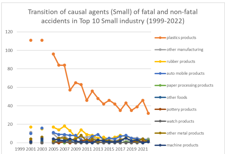
Transition of causal agents (Small) of fatal and non-fatal accidents as code no. 164 injection molding machine in Small Industry (1999-2022)
