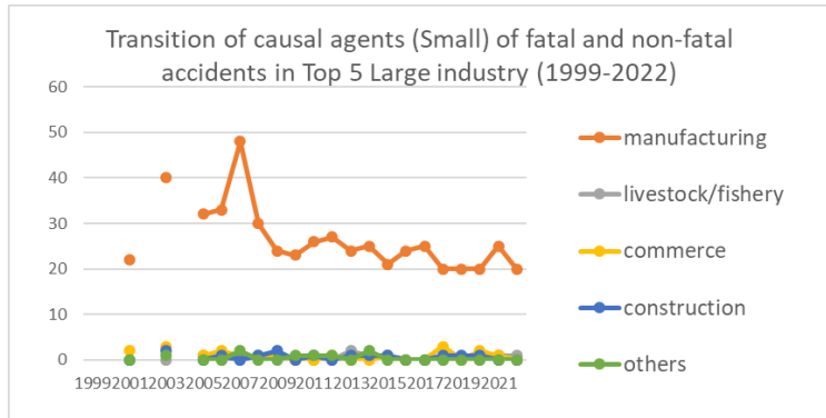
Transition of causal agents (Small) of fatal and non-fatal accidents as code no. 167 industrial robot in Large industry (1999-2022)
