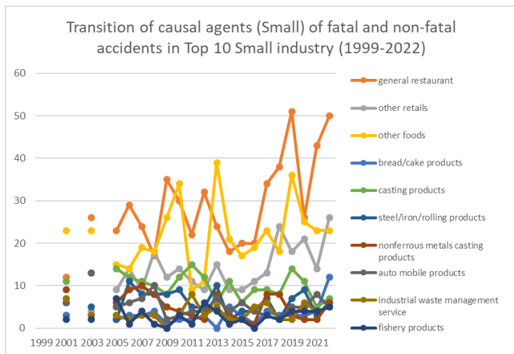
Transition of causal agents (Small) of fatal and non-fatal accidents as code no. 341 kiln, caldron in Small Industry (1999-2022)
