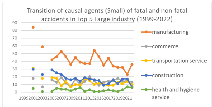
Transition of causal agents (Small) of fatal and non-fatal accidents as code no. 363 human power machine in Large industry (1999-2022)
