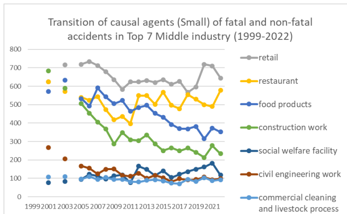
Transition of causal agents (Small) of fatal and non-fatal accidents as code no. 364 hand tool in Middle Industry (1999-2022)
