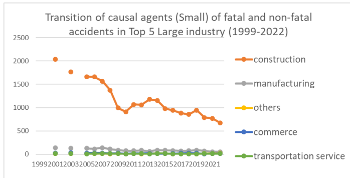
Transition of causal agents (Small) of fatal and non-fatal accidents as code no. 411 scaffolding in Large industry (1999-2022)
