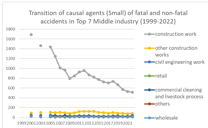
Transition of causal agents (Small) of fatal and non-fatal accidents as code no. 415 roof, beam, haze, crossbeam, principal rafter in Middle Industry (1999-2022)
