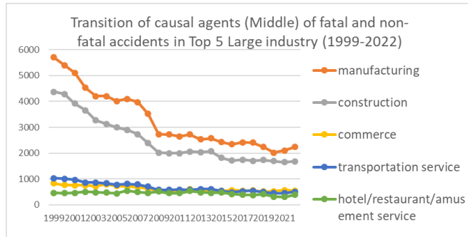
Transition of causal agents (Middle) of fatal and non-fatal accidents as code no. 52 materials in Large industry (1999-2022)
