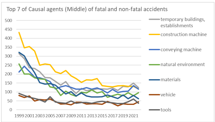
Transition of Top 7 of Causal agents (Middle) of fatal and non-fatal accidents in 030106 road construction work in Japan (1999-2022)
