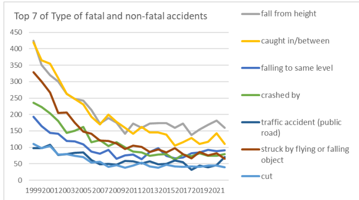
Transition of Top 7 of Type of fatal and non-fatal accidents in 030106 road construction work in Japan (1999-2022)
