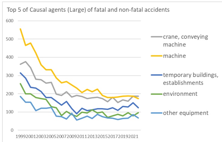
Transition of Top 5 of Causal agents (Large) of fatal and non-fatal accidents in 030106 road construction work in Japan (1999-2022)
