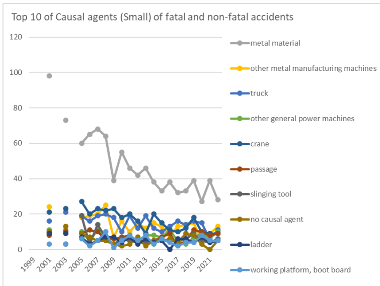
Transition of Top 10 of Causal agents (Small) of fatal and non-fatal accidents in 011009 other steel products in Japan (1999-2022)
